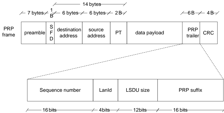
Figure 5. PRP Frame
