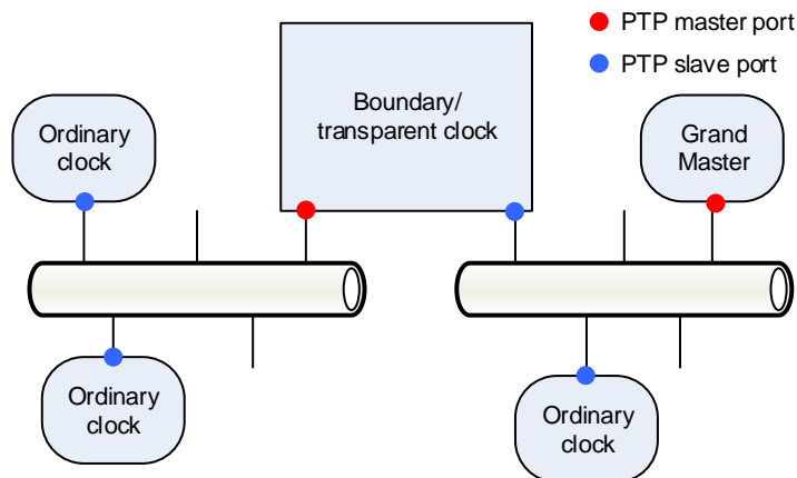
Figure 6. PTP Architecture
